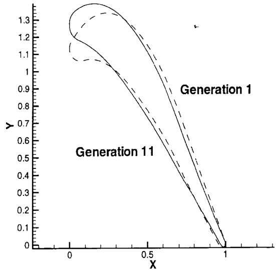
Fig. 9 Best designs for generations 1 and 11 when using penalty function with SQP, minimum thickness distribution constraint, and B-spline geometry perturbation.
