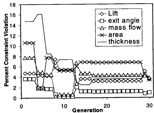
Fig. 6 Violation of constraints when using penalty function and minimum thickness distribution constraint.
