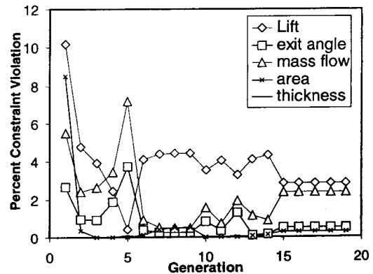
Fig. 10 Violation of constraints when using penalty function with SQP, minimum thickness distribution constraint, and B-spline geometry perturbation.
