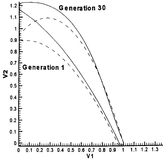
Fig. 7 Best designs for generations 1 and 30 when using penalty function with SQP and minimum thickness distribution constraint.
