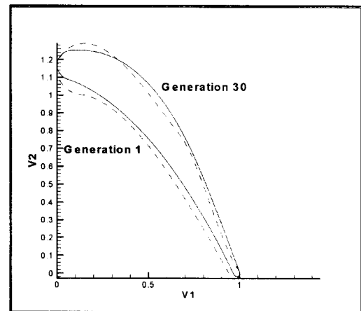
Figure 4. Best designs for generations 1 and 30 when using penalty function and thickness constraint.
