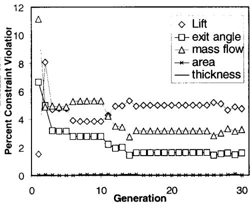
Figure 7. Violation of constraints when using penalty function with SQP and minimum thickness distribution constraint.
