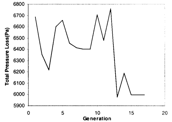
Figure 10. Convergence history of total pressure loss for best designs when using penalty function with SQP, minimum thickness distribution constraint, and B-spline geometry perturbation.
