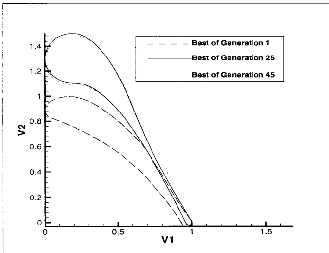
Figure 2. Best designs for generations 1, 25, and 30 when using penalty function only and without minimum thickness distribution constraint.
