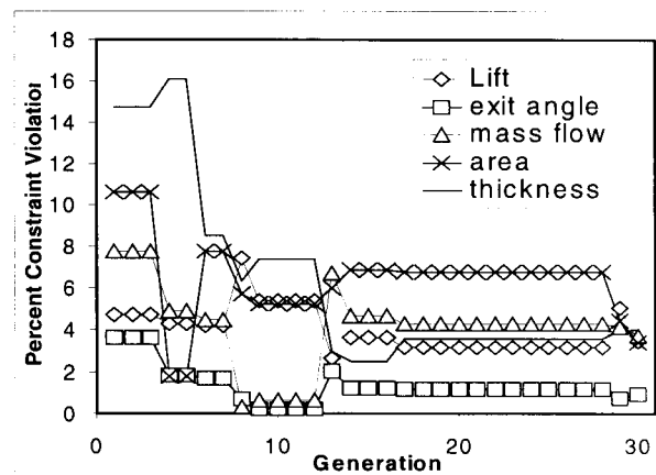
Figure 5. Violation of constraints when using penalty function only and minimum thickness distribution constraint.
