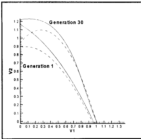
Figure 6. Best designs for generations 1 and 30 when using penalty function with SQP and minimum thickness distribution constraint.
