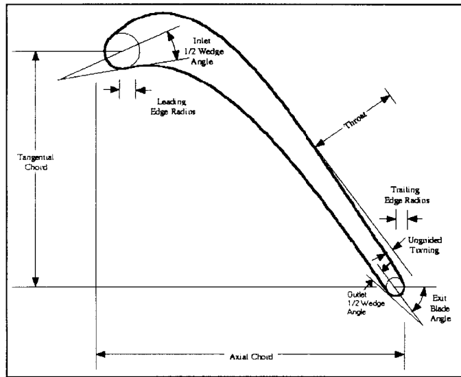
Figure 1. Basic airfoil parameterization.
