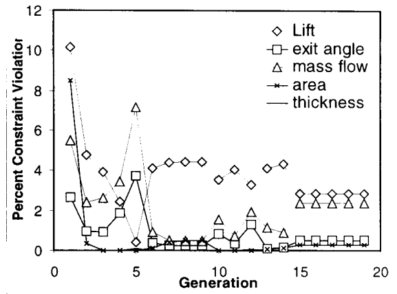
Figure 9. Violation of constraints when using penalty function with SQP, minimum thickness distribution constraint, and B-spline geometry perturbation.
