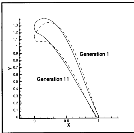
Figure 8. Best designs for generations 1 and 11 when using penalty function with SQP, minimum thickness distribution constraint, and B-spline geometry perturbation.
