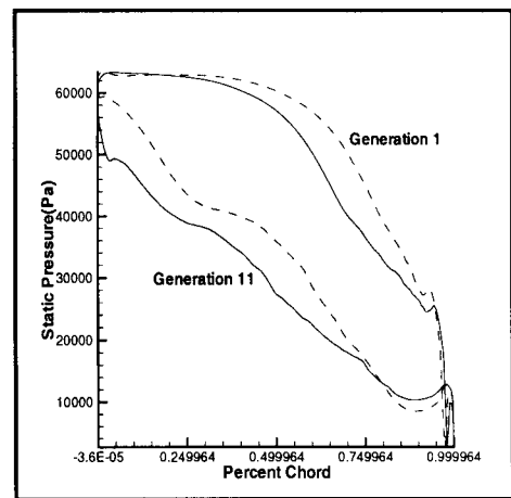
Figure 11: Static pressure distribution for best design of generation 1 and generation 11 when using penalty function with SQP, minimum thickness distribution constraint, and B-spline geometry perturbation.
