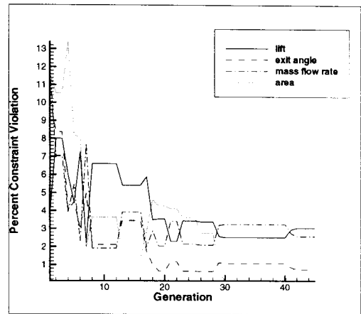
Figure 3. Violation of constraints when using penalty function only and without minimum thickness distribution constraint.
