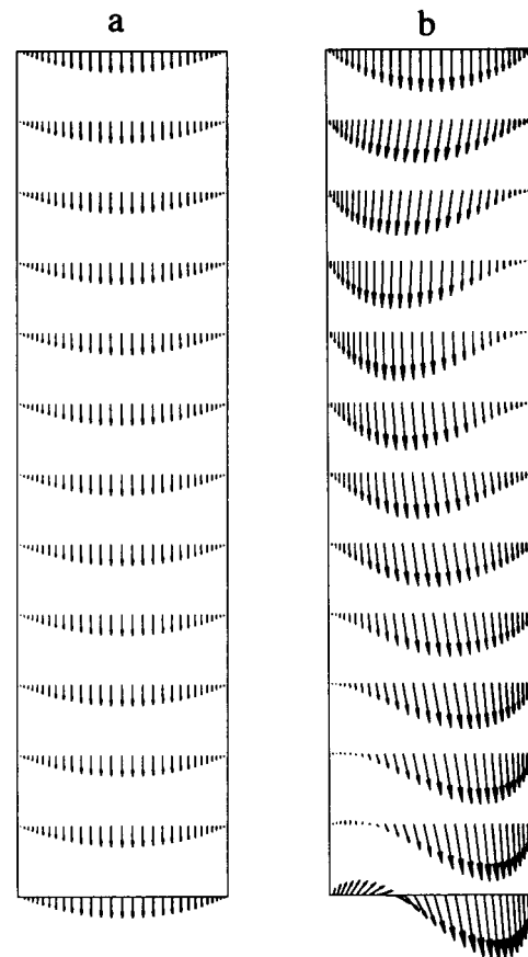
FIGURE 9 Velocity vector fields in a vertical channel; (a) no electric field, (b) 28000 Volts applied between the walls, constant viscosity and sine wave charge distribution along the left vertical wall.
