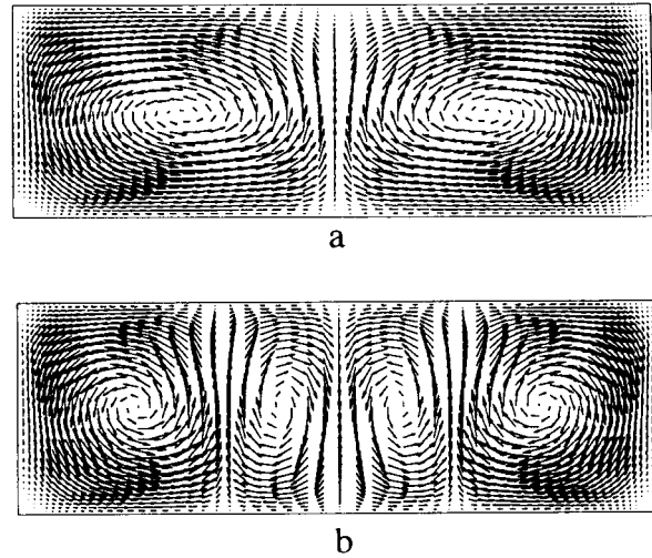
FIGURE 2 Velocity vector fields in a closed container; (a) no electric field, (b) 5600 Volts applied between the top and bottom and uniform charge injection at the bottom wall.
