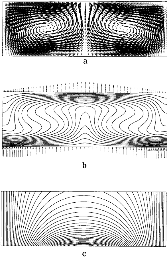
FIGURE 8 Container with 5600 Volts applied between the top and bottom, constant viscosity and sine wave charge distribution at the bottom wall; (a) velocity vector field, (b) isotherms and surface heat fluxes, (c) electric charge densities. (See color plate V.)
