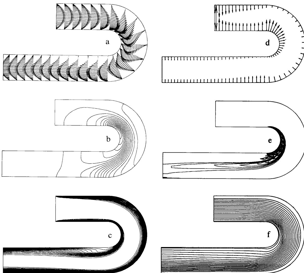
FIGURE 11 U-shaped channel with 500 Volts applied between the walls; (a) velocity vector field, (b) isobars, (c) isotherms, (d) surface heat flux distribution, (e) electric charge distribution, (f) electric potential field. (See color plate VII.)
