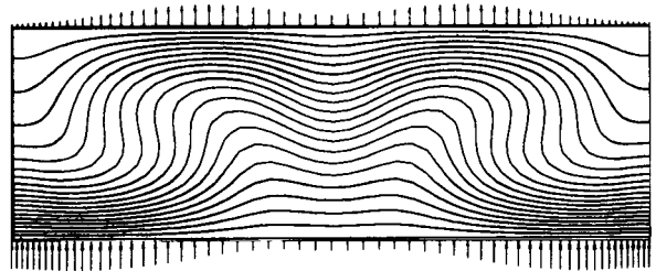
FIGURE 5 Electric charge densities in a closed container (top cold and bottom hot) with 5600 Volts applied between the top and bottom and uniform charge injection at the bottom wall. (See color plate III.)
