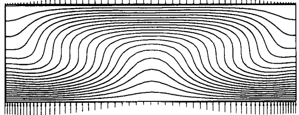
FIGURE 7 Isotherms and surface heat fluxes in a closed container with 5600 Volts applied between the top and bottom, uniform charge injection at the bottom wall and charge-dependent variable viscosity; (a) (\eta/\eta_0)_{\max} = 1.75 , (b) (\eta/\eta_0)_{\max} = 2.0 . (See color plate IV.)
