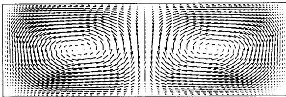
FIGURE 6 Velocity vector fields in a closed container with 5600 Volts applied between the top and bottom, uniform charge injection at the bottom and charge-dependent variable viscosity; (a) (\eta/\eta_0)_{\max} = 1.75 , (b) (\eta/\eta_0)_{\max} = 2.0 .
