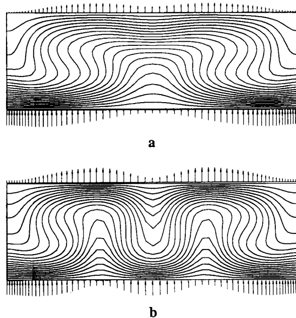
FIGURE 3 Isotherms and surface heat fluxes in a closed container (top cold and bottom hot); (a) no electric field, (b) 5600 Volts applied between the top and bottom and uniform charge injection at the bottom. (See color plate I.)
