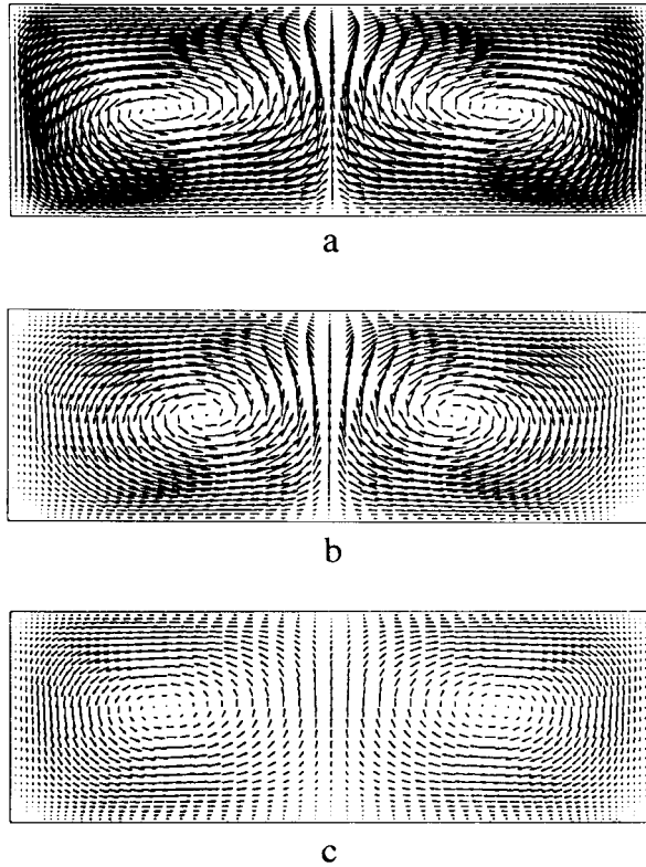
FIGURE 1 A demonstration of an electro-thermal convection in a closed container (top cold and bottom hot) with an electric potential difference imposed between the top and bottom. Velocity vector fields for; (a) combined thermal convection and electroconvection, (b) thermal convection alone, (c) electroconvection alone.
