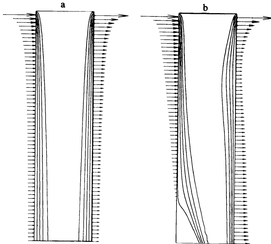
FIGURE 10 Isotherms and surface heat fluxes in a vertical channel; (a) no electric field, (b) 28000 Volts applied between the walls, constant viscosity and sine wave charge distribution along the left vertical wall. (See color plate VI.)
