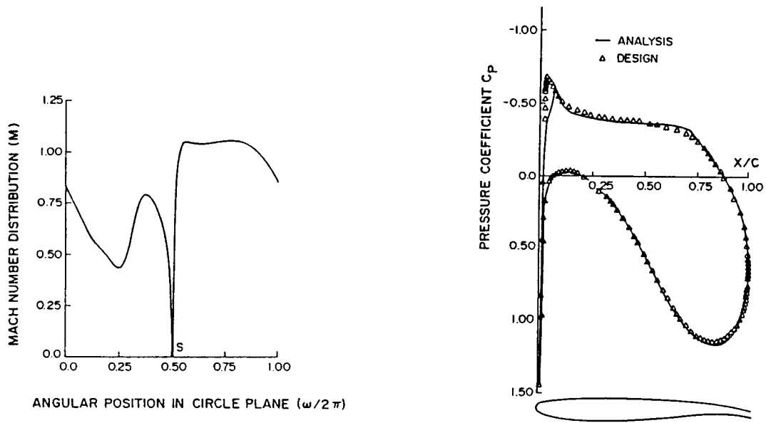
Fig. (10) Shock-free compressor blade and its corresponding Mach number and pressure distributions ( M_1 = 0.680 , M_2 = 0.570 , \theta_1 = -40.0^\circ , \theta_2 = -5.624^\circ , solidity = 0.792)
