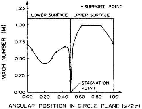
Fig. (5) Typical input subsonic-sonic Mach number distribution for a blade having a cusped trailing edge
