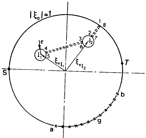
Fig. (4) Blade subsonic-sonic boundary in the circle plane
