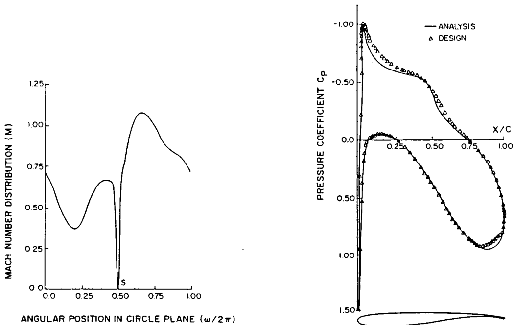
Fig. (9) Shock-free compressor blade and its corresponding Mach number and pressure distributions ( M_1 = 0.750 , M_2 = 0.600 , \theta_1 = -30.0^\circ , \theta_2 = -7.82^\circ , solidity = 0.85)
