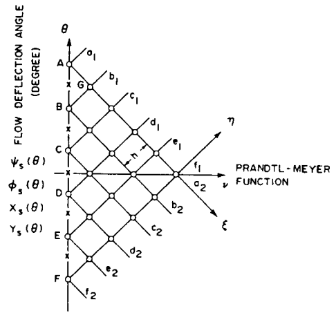
Fig. (7) Computation of the supersonic flow field in the hodograph plane using the method of characteristics
