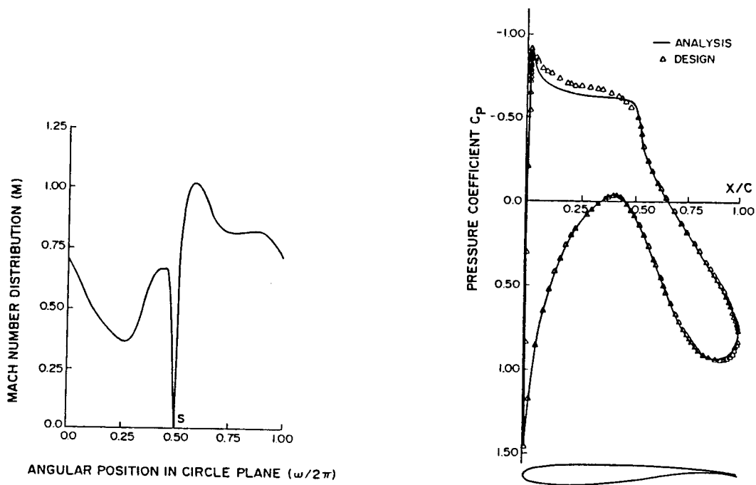
Fig. (8) Shock-free compressor blade and its corresponding Mach number and pressure distributions ( M_1 = 0.750 , M_2 = 0.652 , \theta_1 = -35.0^\circ , \theta_2 = -3.17^\circ , solidity = 1.0)
