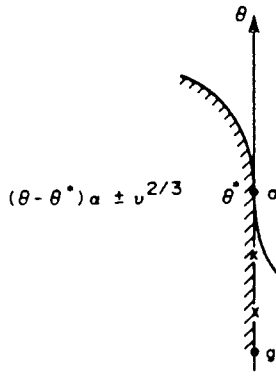
Fig. (3) Local structure of the blade contour near the sonic points a and b
