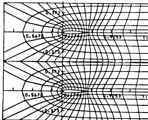
C-TYPE GRID
