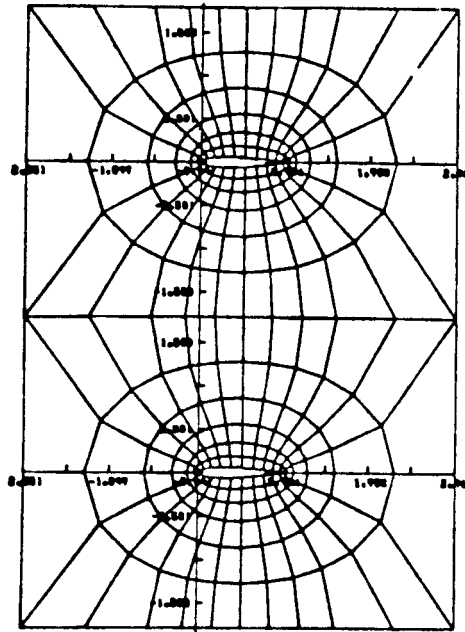
O-TYPE GRID
