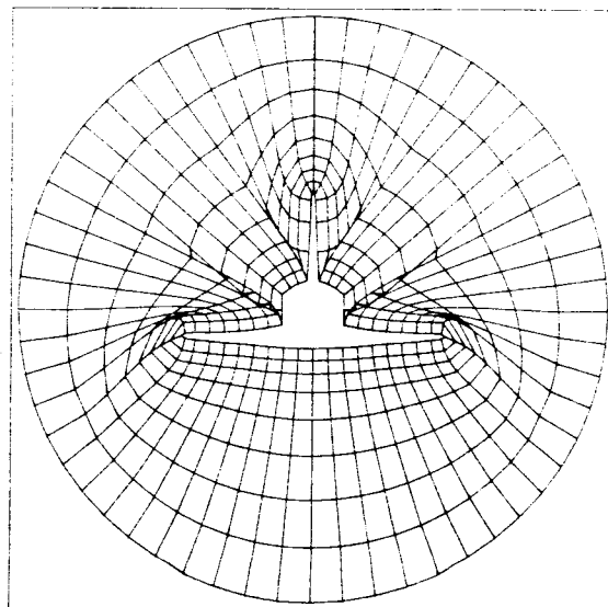
Fig. 6 Nonoptimal O-type grid for Space Shuttle cross section, grid size 56 x 8.
