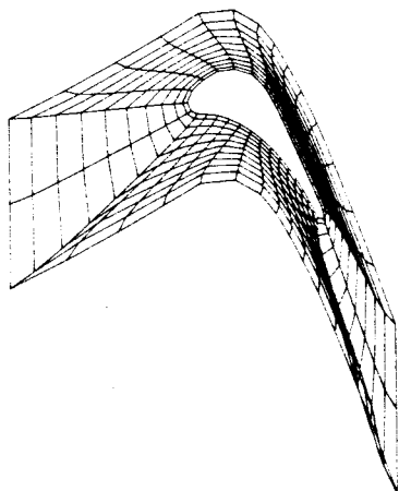
Fig. 4 Nonoptimal periodic O-type grid for MIT turbine airfoil cascade, gap-to-chord ratio = 1.0, grid size 32 x 10.
