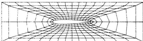
Fig. 2 Nonoptimal periodic O-type grid for NACA 0012 airfoil cascade, gap-to-chord ratio = 1.0, grid size 32 x 8.
