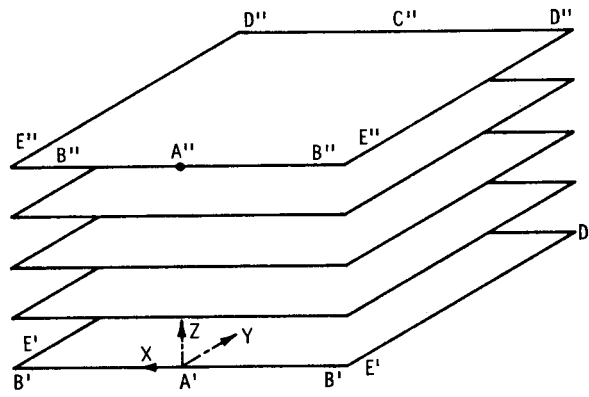
Figure 2. - Computational space.
