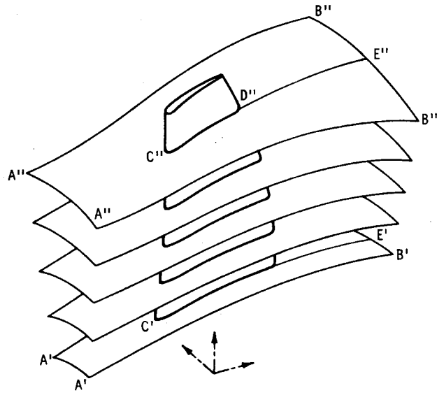
Figure 1. - Physical space.
