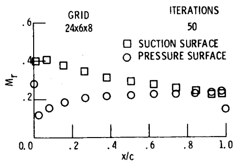
Figure 5. - Subsonic rotor.
