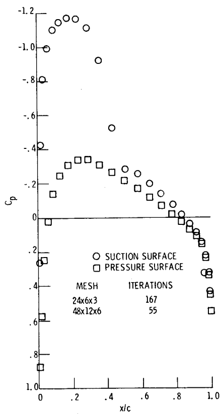
Figure 6. - Transonic rotor.
